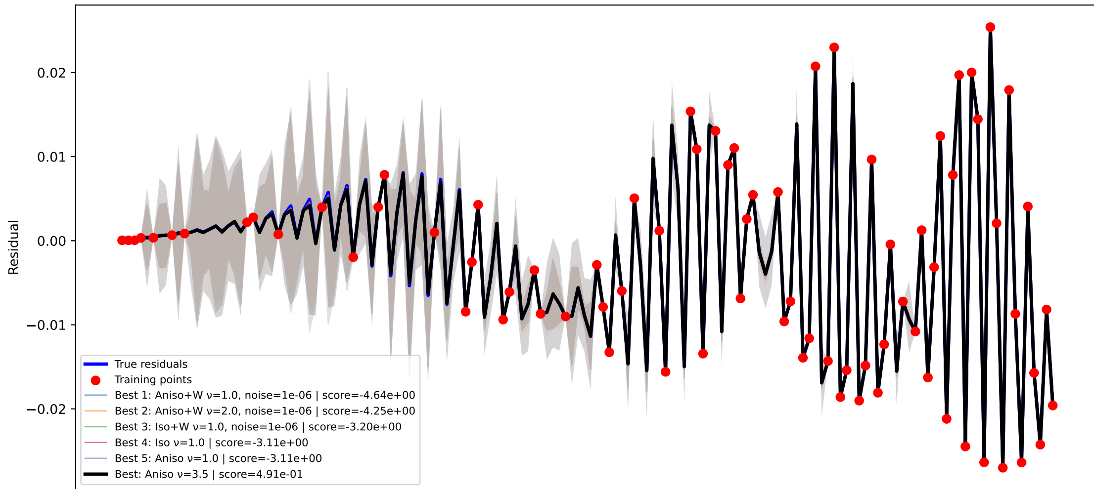
GPR kernel comparison node=43 RMSE=1.290e-04, train RMSE=1.899e-11
